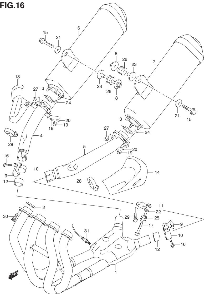
FIG.16 (C-8) MUFFLER
