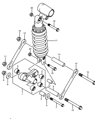
FIG.59 REAR CUSHION LEVER (K-3)
