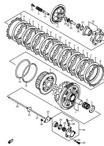
FIG.23 CLUTCH (D-2)
