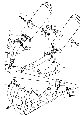
FIG.16 MUFFLER (C-8)
