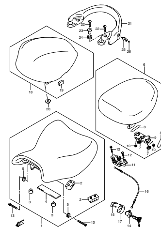
FIG.51A SEAT (MODEL K9) (J-4)
