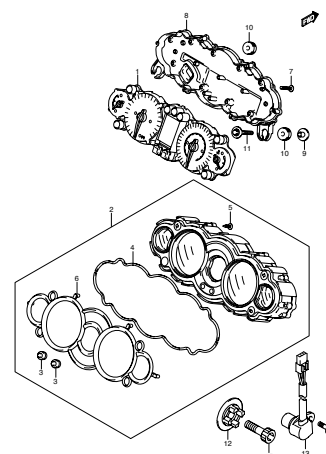
FIG.30 SPEEDOMETER (E-2)
