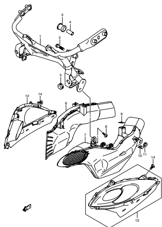
FIG.48B SIDE COWLING (MODEL L0) (H-7)
