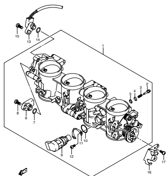
FIG.13 THROTTLE BODY (C-5)
