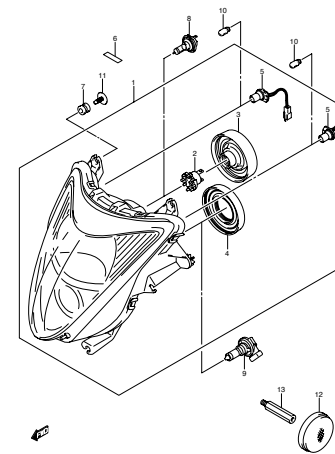
FIG.31 HEADLAMP (E-3)
