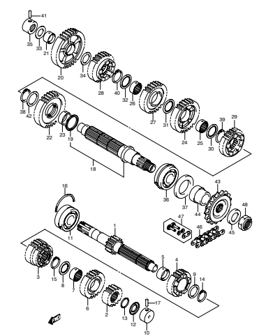
FIG.24 TRANSMISSION (D-3)
