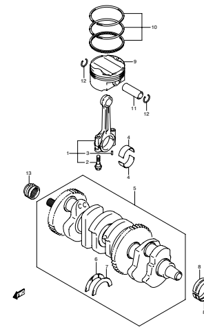
FIG.8 CRANKSHAFT (B-12)
