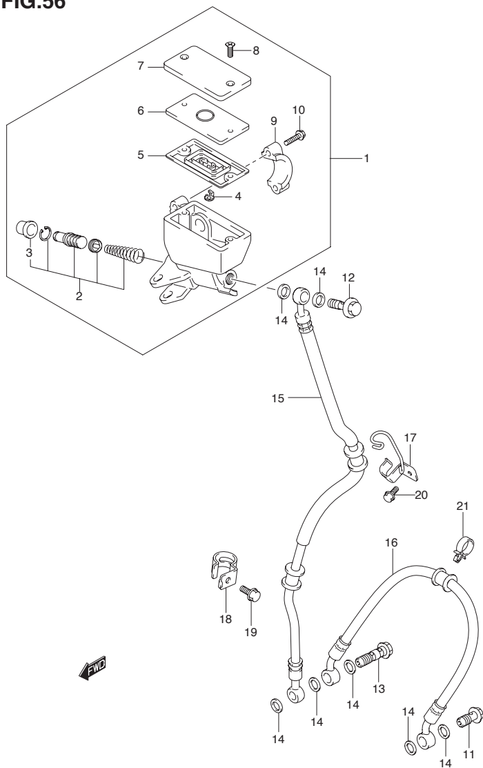
GSX1300RK8 E02_056 FRONT BRAKE HOSE-C
