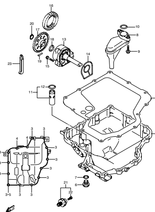
FIG.7 OIL PAN/OIL PUMP (B-11)
