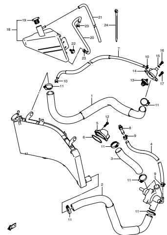
FIG.21 RADIATOR HOSE (C-13)
