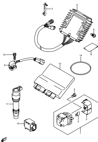
FIG.28 ELECTRICAL (D-10)
